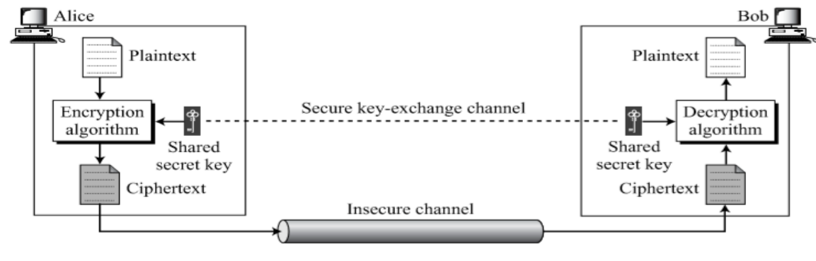
Figure 3.1 General idea of symmetric-key cipher
