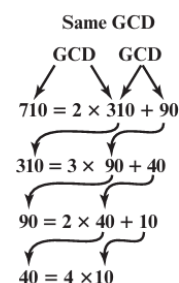
Figure 2.3 Euclidean Algorithm Example: \gcd(710, 310)
